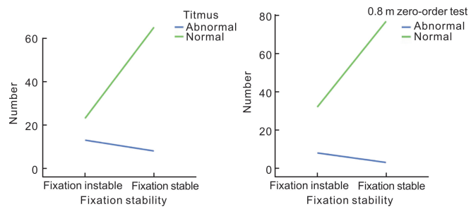
Figure 9 Correlation between fixation stability and near stereoacuity was showed above. When the subjects showed instable fixation, subjects tend to show abnormal results in near stereoacuity tests (Titmus and 0.8 m zero-order test).
