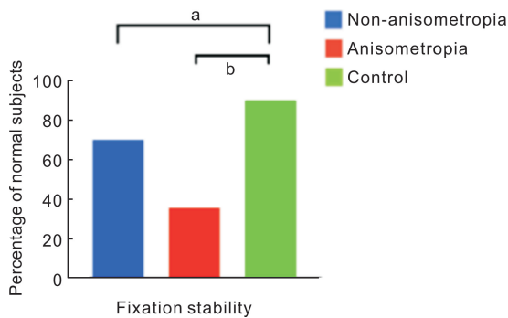
Figure 7 Bar graph showed the percentages of subject with stable fixation.
