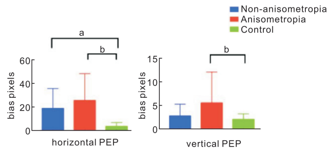
Figure 5 Bar graph showed the average horizontal and vertical bias pixels of each groups. Error bars showed the standard deviation (SD).
