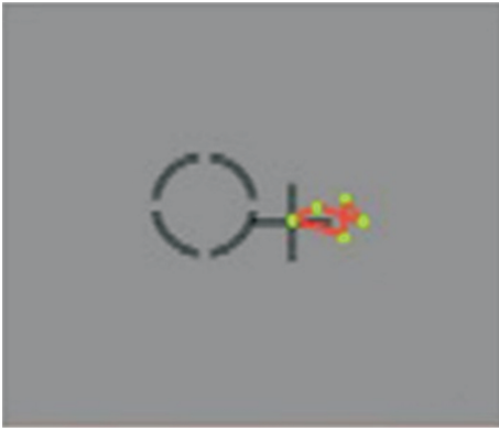
Figure 6 Picture above depicted the moving trace (cross) of one subject with instable fixation. The green dots represented the center of the cross, and the red lines depicted the moving trace of the cross.
