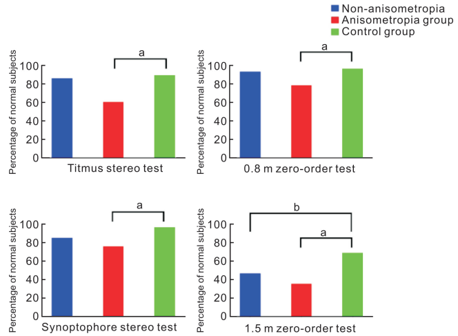
Figure 8 Bar graph showed the percentage of normal subjects in near and far stereoacuity tests within groups.
