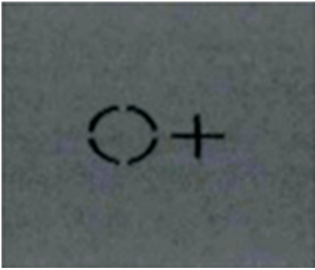
Figure 2 Picture above showed example of the PEP test. Subjects were able to see a cross with their left eye and a circle in right eye.
