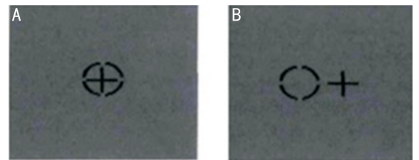
Figure 4 A: The results of normal subjects in PEP test. Subjects with normal PEP were able to move the cross into the middle of the circle; B: The result of one subject with abnormal PEP. Subjects with abnormal PEP would fail to move the cross into the middle of the circle while they thought they did.
